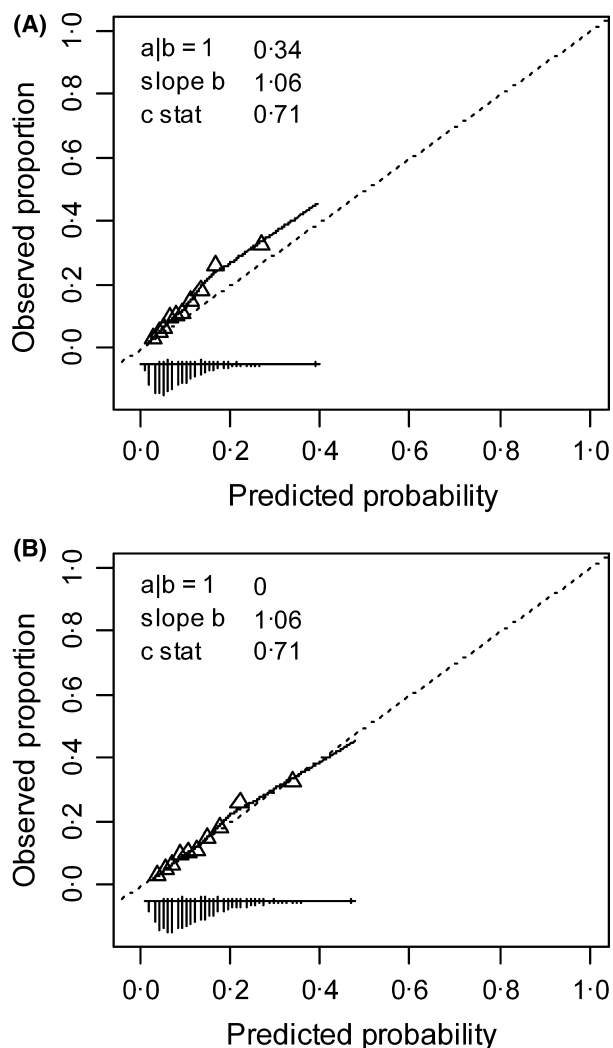
Fig 1. Validation plots for the prediction model of an international normalised ratio \geq 4.5 . (A) the calibration-in-the-large (a|b) was 0.34 and the calibration slope (slope b) was 1.06 before correction; (B) after correction for the calibration-in-the-large, the calibration-in-the-large was 0 and the calibration slope was 1.06. The distribution of predicted risks is shown at the bottom of the graphs. Triangles indicate the observed proportions by quintiles of predicted risks.
