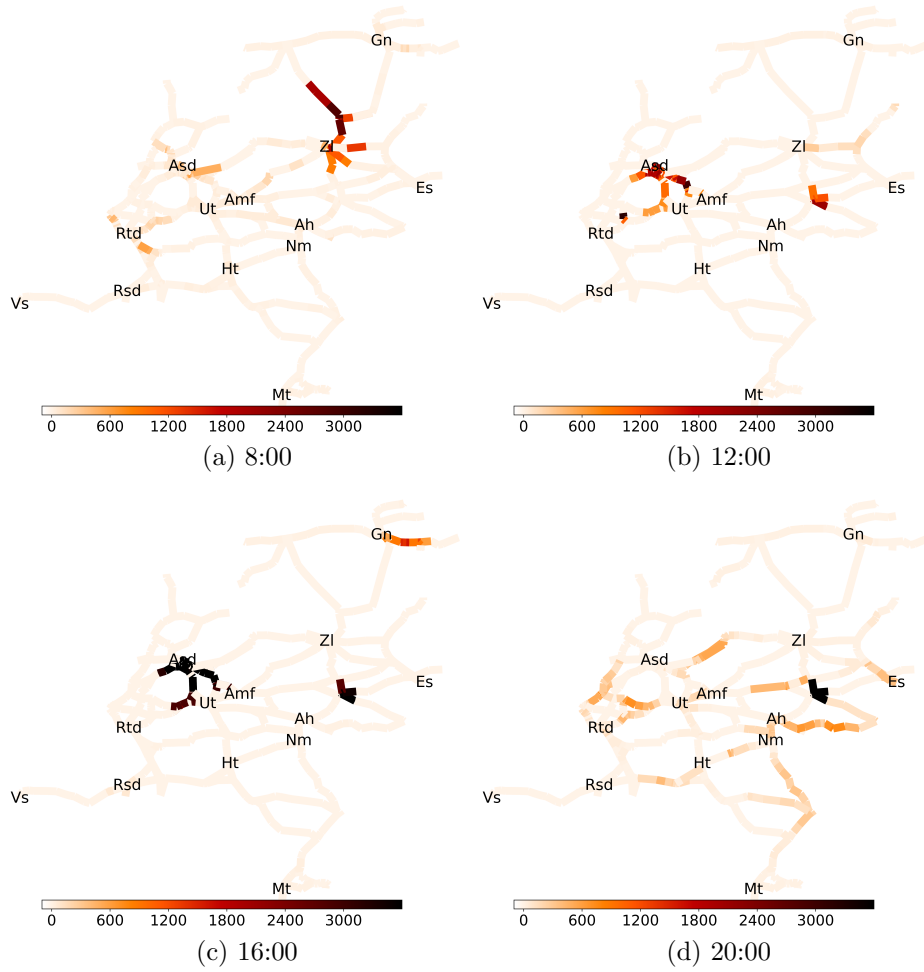
Figure 5: Delay evolution on January 18, 2018, a day with a severe storm that caused the deliberate shutdown of a large part of the network.
