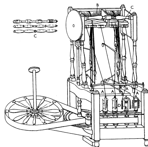
Arkwright's spinmachine
