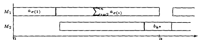
Figure 4. The position of the partition job J_{k^*} .
