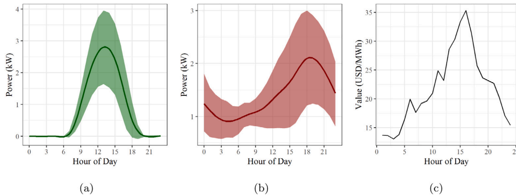
Fig. 4. Generation (a) and consumption (b) of households and average ERCOT RTLM (c) per hour-of-day. Shaded areas indicate one standard deviation (Except for (c), whose standard deviations were too large to display with averages).
