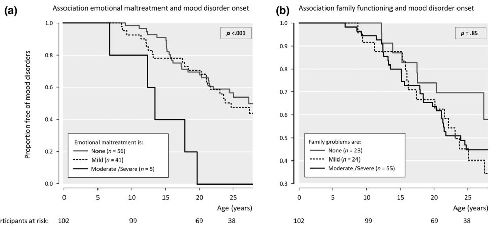
Figure 1. Emotional maltreatment/family functioning and mood disorder onset. The total (continuous) CTQ and QFP scores are used for the Cox regression analyses. In order to make the associations visible with Kaplan–Meier curves in this figure, total scores were categorized into three severity categories based on Bernstein et al. (2003) for the CTQ and on the norm scores of the QFP.
