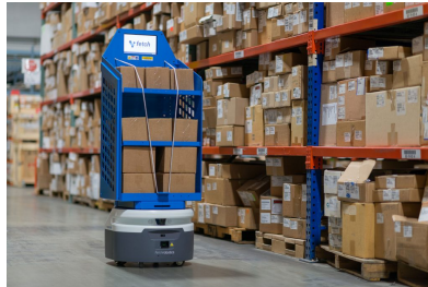
Figure 1.6: Pick-Support AMR (Source: Fetch Robotics)
