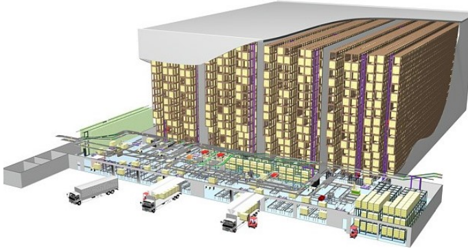
Figure 2.4: Automated high-bay warehouse for pallets with aisle-captive cranes (De Koster, 2015)
