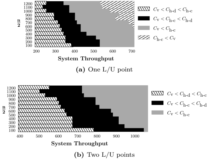
Figure 3.18: Summary of the cost comparison of the three systems
