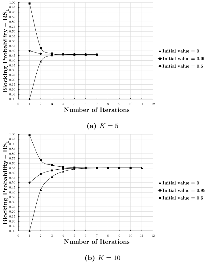
Figure 3.12: Number of iterations the algorithm needs to converge
