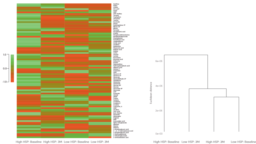
Figure 5 – HSP level and L-glutamine supplementation affects metabolic phenotypes. A: heat map of the absolute levels of all 83 metabolites for high HSP: baseline, high HSP: 3-month follow-up (3M), low HSP: baseline and low HSP: 3M. The pooled group high HSP at baseline is distinct from the other groups. B: dendrogram showing the hierarchical clustering using the Euclidean distance with average linkage for all four groups.
