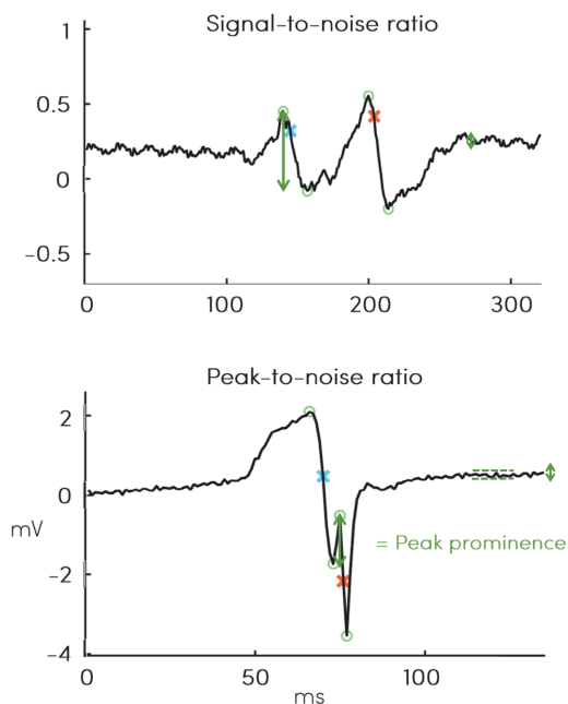
Supplemental figure 2 – signal-to noise and peak-to-noise ratio. Top: the ratio between the amplitude of the deflection and amplitude of the noise defined the signal-to-noise ratio. Bottom: the ratio between the peak prominence and the amplitude of the noise determined the detection of a new peak and the presence of a new deflection.
