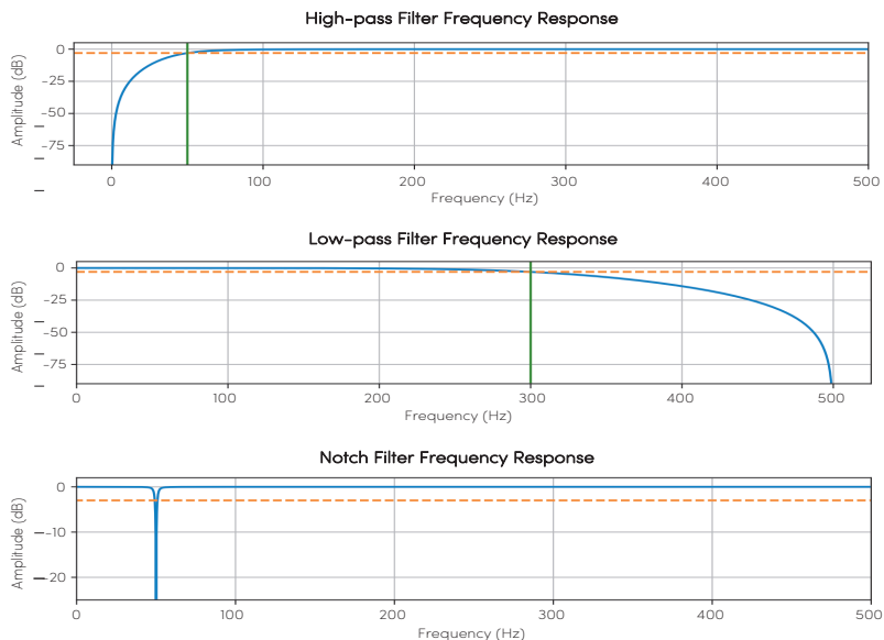
Supplemental figure 1 – Bode plots of the used filters. Upper panel: filter frequency response of IIR Butterworth high-pass filter, 2nd-order with 12 dB/octave roll-off with an exemplary half amplitude (-3 dB) cut-off frequency of 50 Hz. Middle panel: filter frequency response of IIR Butterworth low-pass filter, 2nd-order with 12 dB/octave roll-off with an exemplary half amplitude (-3 dB) cut-off frequency of 300 Hz. Lower panel: filter frequency response of IIR notch filter at 50 Hz, with a quality factor of 30.
