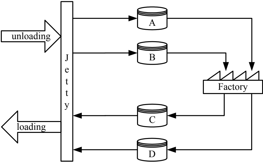
Figure 1: A schematic outline of the loading and unloading process, including jetty, tanks and factory
