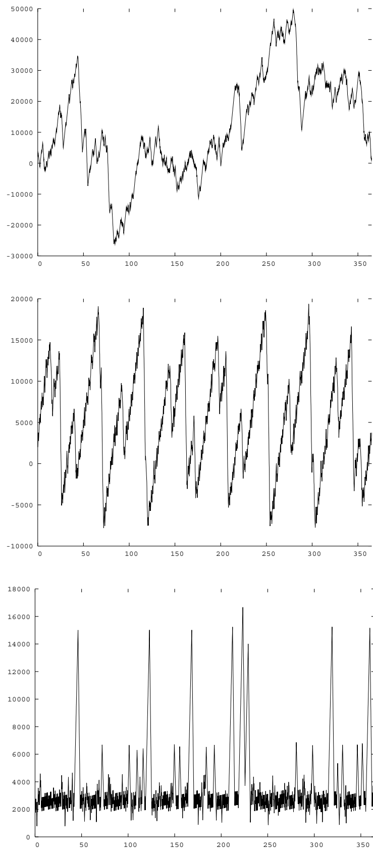
Figure 5: Level of Tank D during one year with uncontrolled (top), equidistant (middle) and stock-controlled process (bottom)
