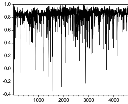
Figure 2 Dynamic conditional correlations
