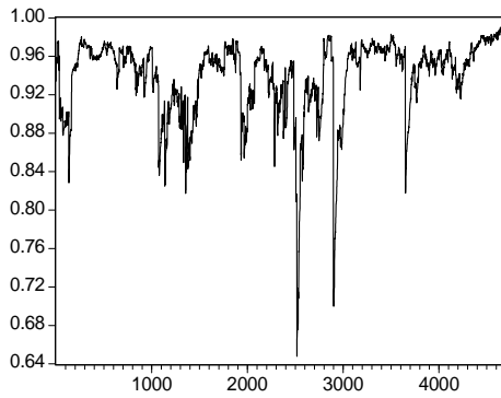
Figure 2 Dynamic conditional correlations
