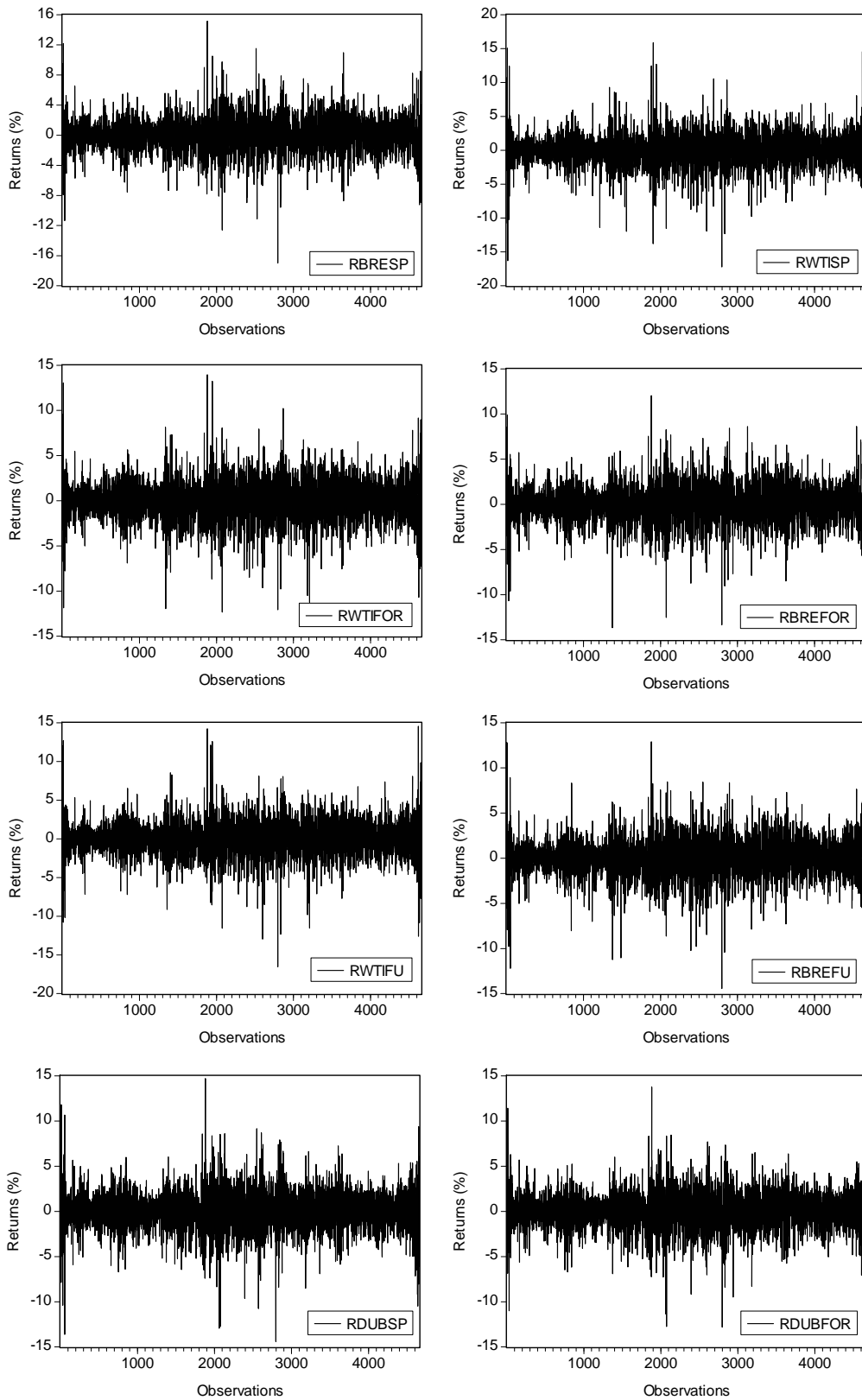
Figure 1 Logarithm of daily spot, forward and futures returns for Brent, WTI and Dubai
