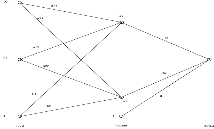
Figure 3. Graph of a neural network
