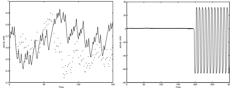
Figure 5. Actual (scaled) data CH95 , \gamma = 4 and orbit data (continuous line) generated by neural network nn(3, 2, 1) . Left panel: time index from 1 to 150; right panel: time index from 1 to 300
