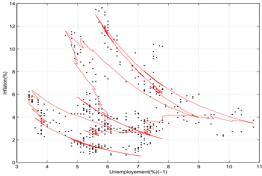
Figure 15. Estimated data of model nn(t) \times nn(x) , with H = 1 , and actual data INFR12
