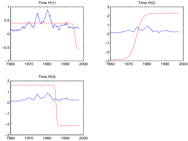
Figure 17. Output of hidden layer cells of nn(t) (case x -network with H = 1 )
