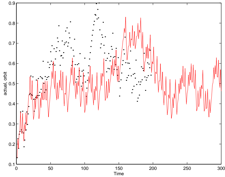
Figure 6. Actual (scaled) data with \gamma = 3.95 and orbit data (continuous line) generated by neural network nn(3, 2, 1)
