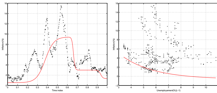
Figure 16. Output of nn(t) (left) and nn(x) (case H = 1 ) (right) compared to actual data INFR12
