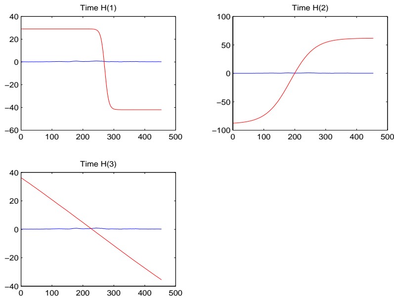
Figure 14. Output of hidden layer cells of t -network nn(t) in case of the x -network with H = 3
