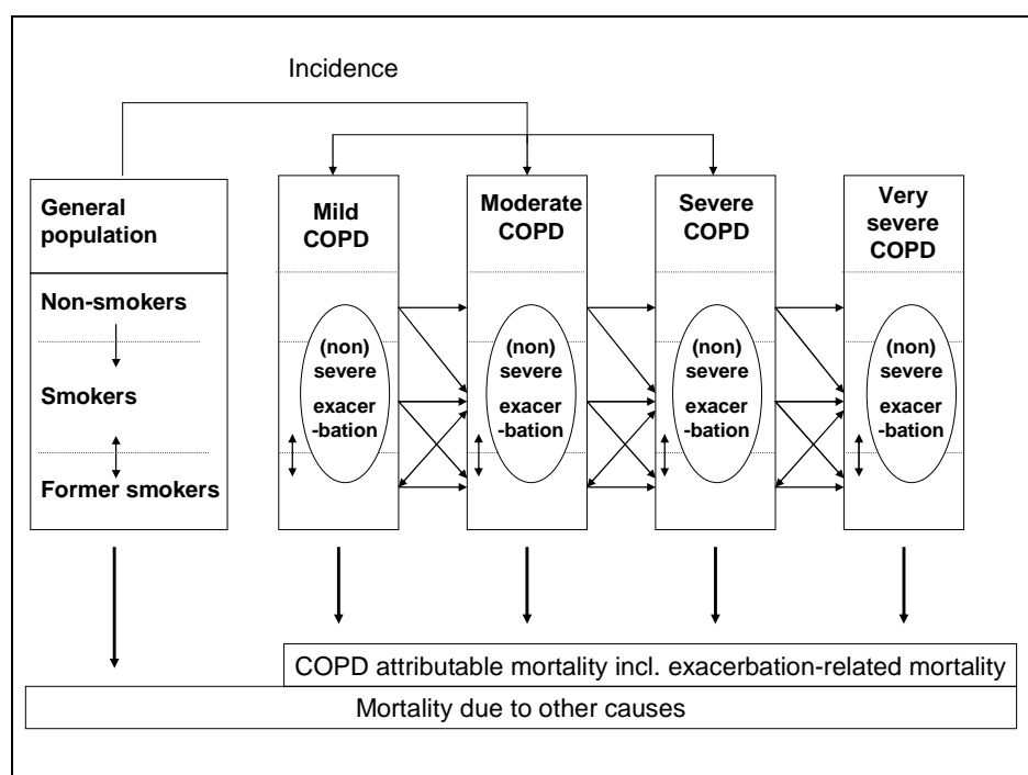
Figure 2.1. Description of the Dutch COPD population model
