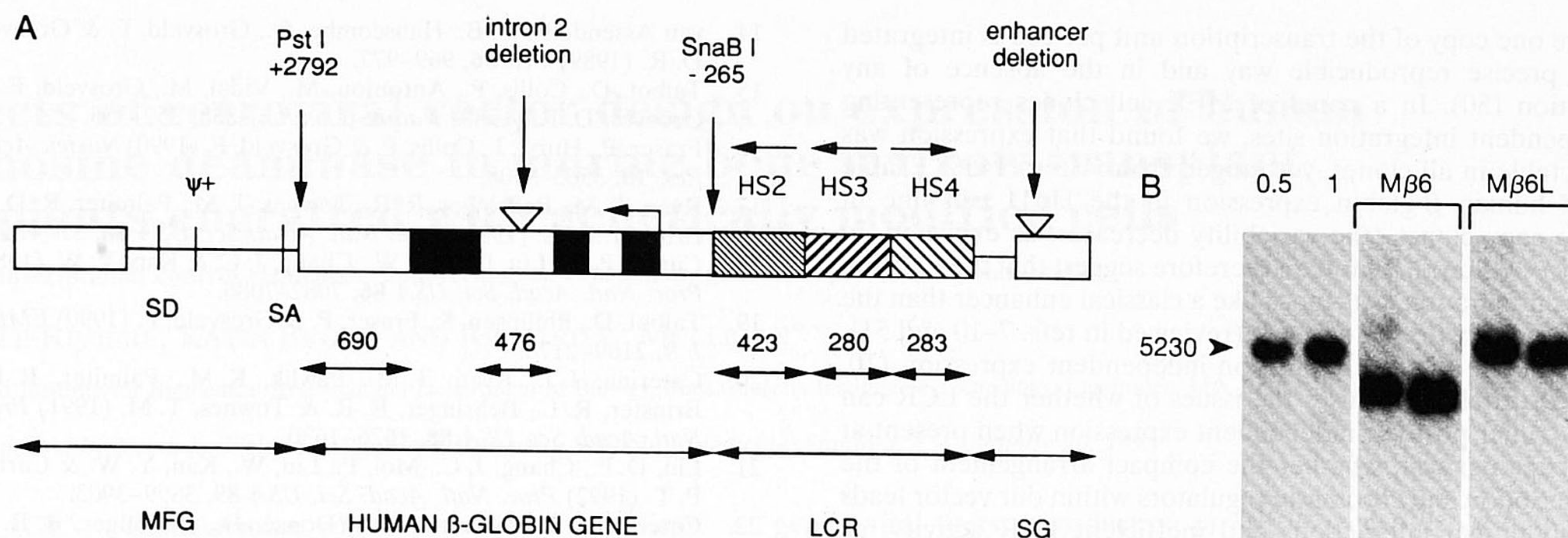
FIG. 5. (A) Schematic representation of the M \beta 6L vector. Black boxes represent the \beta -globin exons. Arrows above the HS boxes indicate their orientations. Numbers below delineated segments represent fragment length in bp. \psi +, packaging signal. White boxes at ends represent LTRs. See text for exact sequences. SD, splice donor; SA, splice acceptor; MFG, 5' sequences derived from the MFG vector; SG, 3' sequences derived from the SG vector. (B) Transmission characteristics of vectors M \beta 6L and M \beta 6, the parent \beta -globin gene vector lacking the LCR fragment. Southern blot analysis is carried out as in the previous figures. Length on left is in bp.
