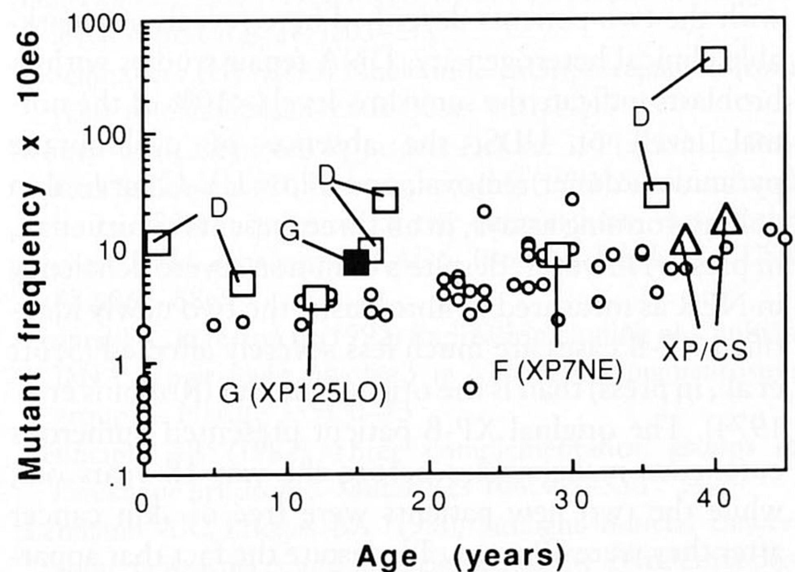
Figure 5 hprt mutant frequency in circulating T-lymphocytes in normal, nonsmoking subjects and in XP patients. Frequency of hprt mutants is set against the age of the donors, who are normal, nonsmoking donors (○), an XP nonsmoker (□), an XP smoker (■), and XPCS1BA and XPCS2BA (△).
