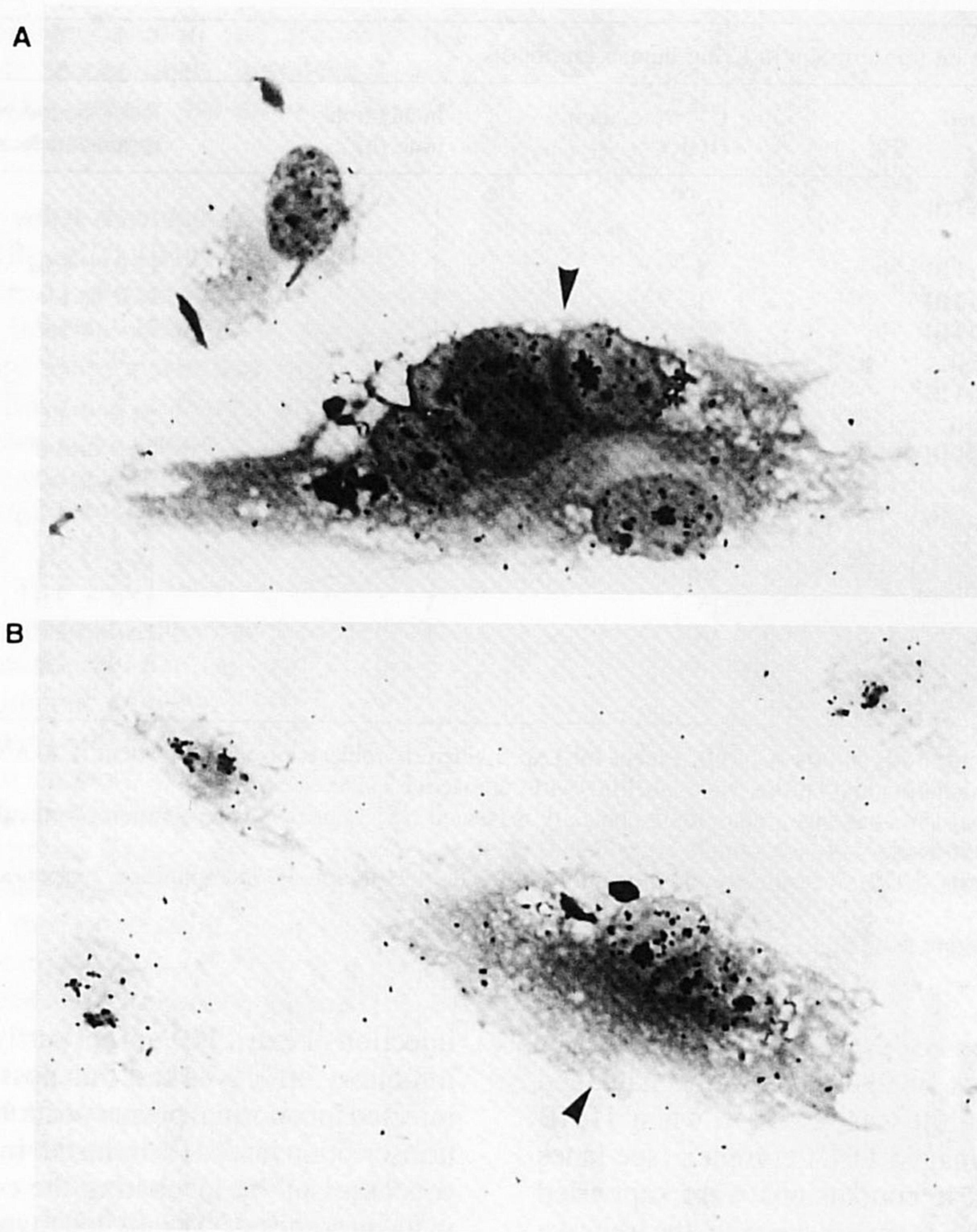
Fig. 6. Effect of TBP on transcription in vivo . Micrograph of C5RO normal (A) and CS-B patient (B) fibroblasts injected (indicated by an arrow) 1 h before UV irradiation ( 16 \text{ J/m}^2 ) showing an increase in the overall RNA synthesis. In each panel, one has to compare the autoradiographic grains above the nuclei of injected cells (indicated by an arrow) with the surrounding nuclei.
