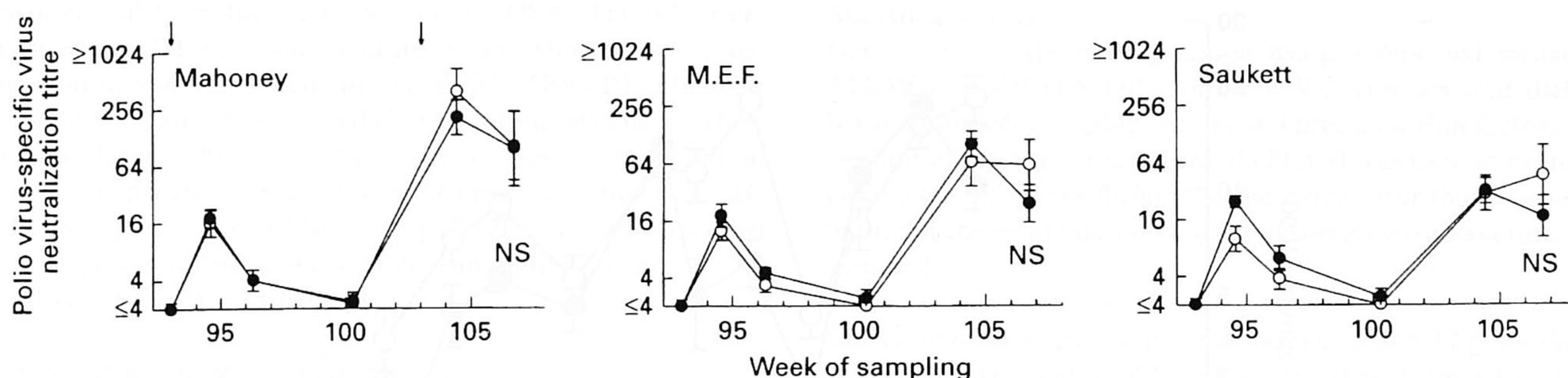
Fig. 4. Virus neutralizing serum antibody titres against polioviruses type 1 (Mahoney), type 2 (MEF) and type 3 (Saukett) in seals fed Atlantic (○) or Baltic (●) herring, after immunization with trivalent polio vaccine. Immunizations are indicated by arrows. Data shown are means \pm s.e.m. NS, Not significant.
