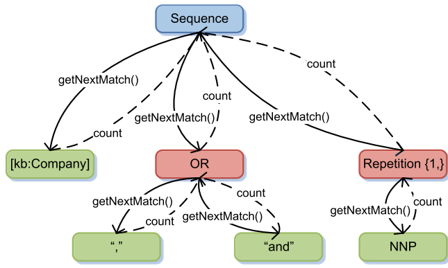
Fig. 3. Rule tree example of Rule 14.
