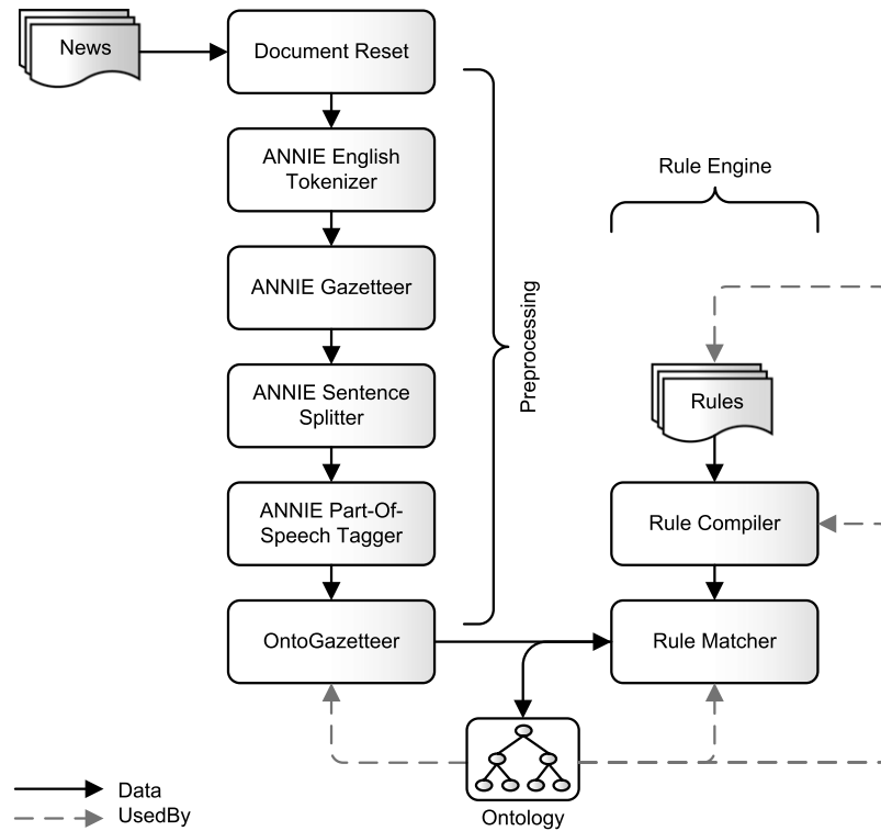
Fig. 1. Overview of the Hermes processing pipeline.
