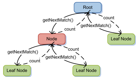
Fig. 2. Rule tree template.
