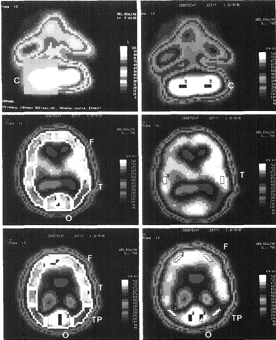
Figure 3.1.1 An example of a SPECT scan (Siemens camera) of a normal control. Figures on the left hand panel: regions of interest drawn with reference to normal anatomy; the boundary of the cerebellar reference slice (C) is defined by activity higher than 70% of the maximum value in this slice. Figures on the right hand panel: 2x4 pixels rectangular ROI's. C=cerebellum, F=frontal, T=temporal, P=parietal, TP=temporo-parietal, O=occipital
