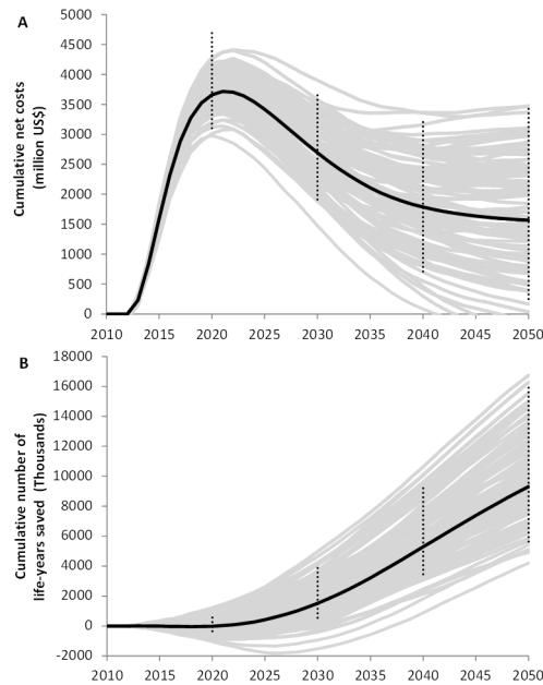
Figure 4. Cumulative net costs and cumulative number of life-years saved of universal testing and immediate ART for all HIV-infected patients (UTT) compared to the current rollout in South Africa of ART at CD4 count \leq 350 cells/ \mu l, as predicted with model D. (A) Cumulative net costs; (B) cumulative number of life-years saved. Grey lines represent 100 individual model runs illustrating stochastic variation; black lines are averages over 1,000 model runs. Error bars reflect ranges due to uncertainty in the parameter values that were quantified based on fitting the model to data. Costs and life-years saved were discounted at an annual rate of 3%. doi:10.1371/journal.pmed.1001534.g004
