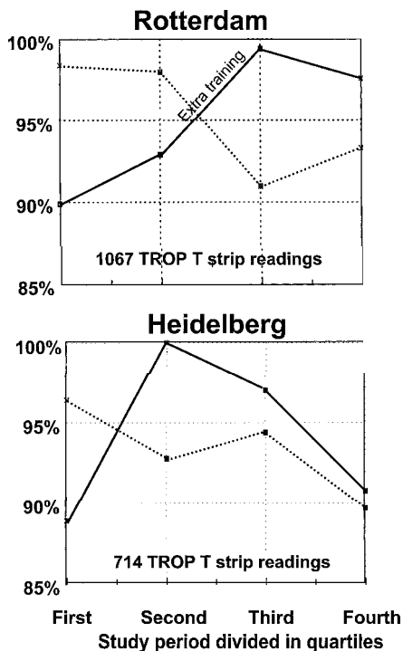
FIG. 3. Learning curve of the analytical sensitivity and specificity of Trop T throughout the study period. The study period was evenly divided in quartiles. ■ Analytical sensitivity. •••• Analytical specificity.
