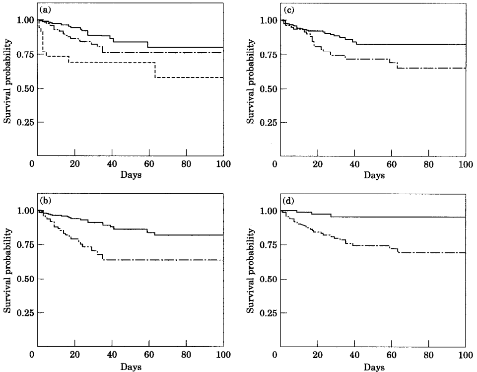
Figure 1. Kaplan–Meier curves for development of MRSA infection among colonized patients by: (a) hospital departments [(—) medicine; (·····) intensive care; (---) surgery]; (b) surgical wounds [(—) without; (---) with]; (c) pressure ulcers [(—) without; (---) with]; (d) intravenous catheters [(—) without; (---) with]. The 'survival probability' (y-axis) is the proportion of patients who are free of MRSA infection. The curves shown are censored at 100 days. By this time only 26 patients were still at risk and only three subsequently developed infection.
