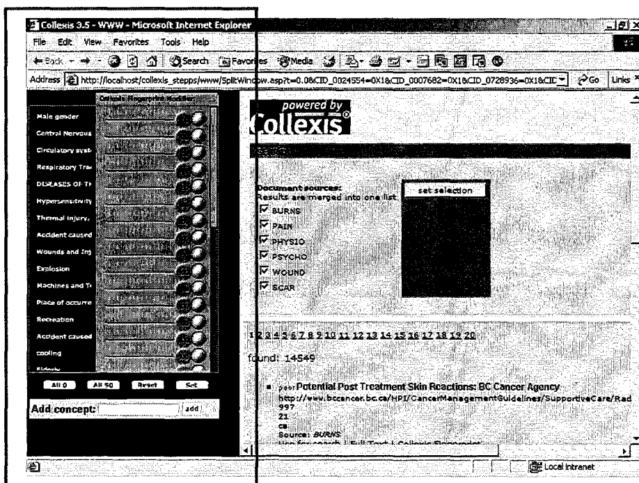
FIGURE 3. Presentation of the matching results screen The frame highlights the Fingerprint modifier area of the window.
