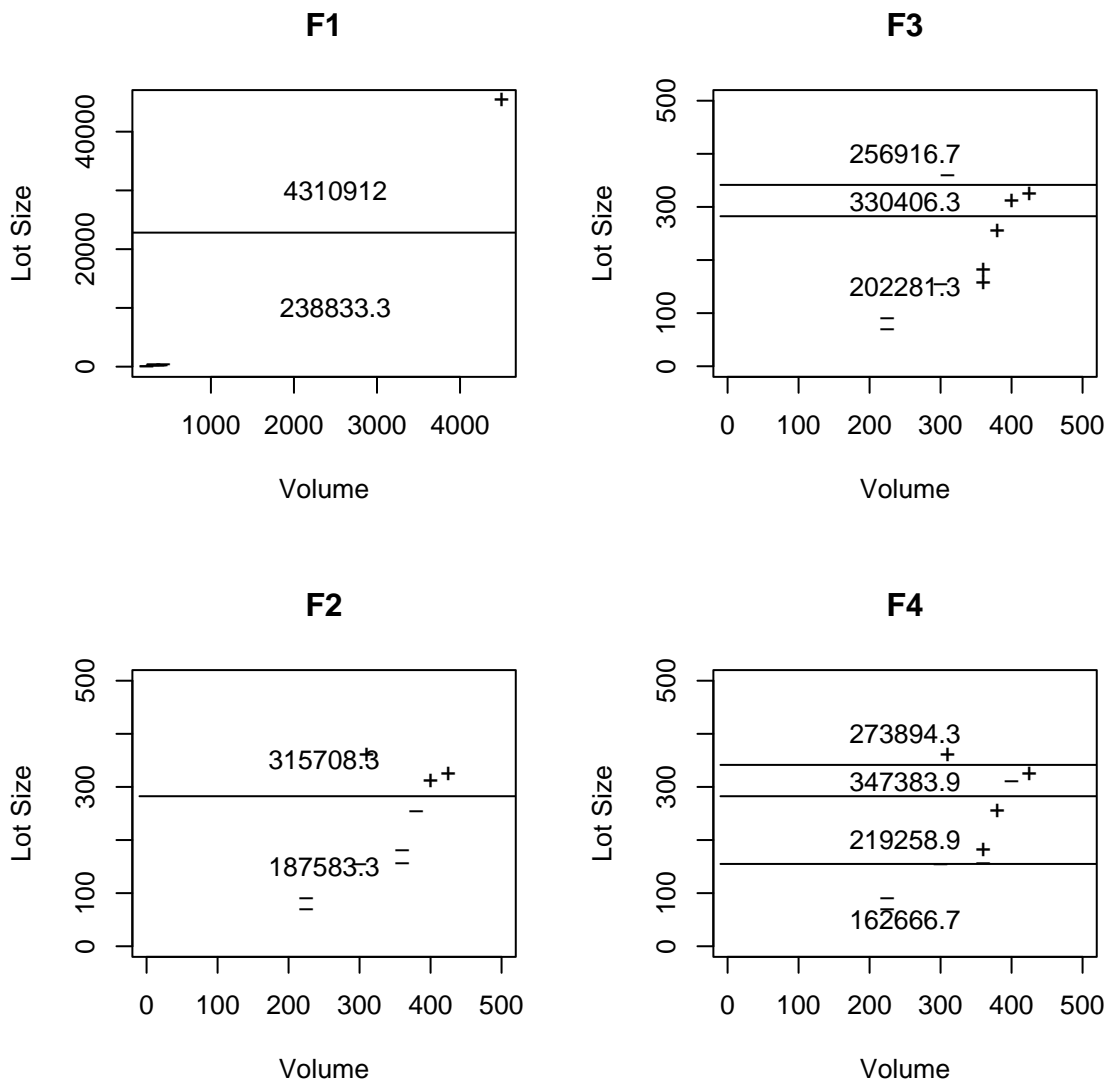
Figure 2: LSBoost process
