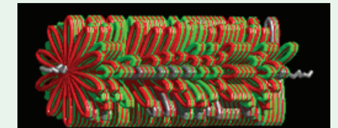
Fig. 8A: Starting configuration with the form and size of a metaphase chromosome.
