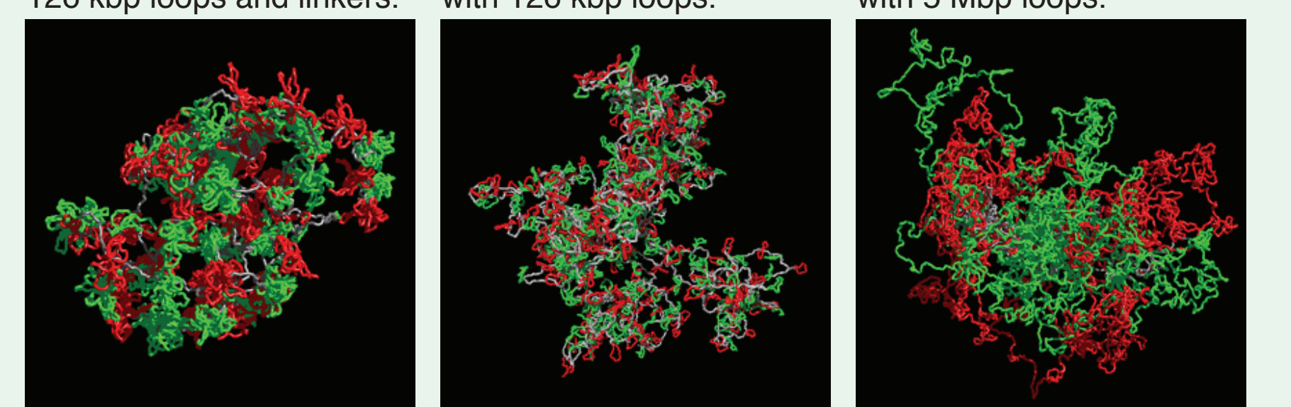
Fig. 8B: MLS model with 126 kbp loops and linkers.
