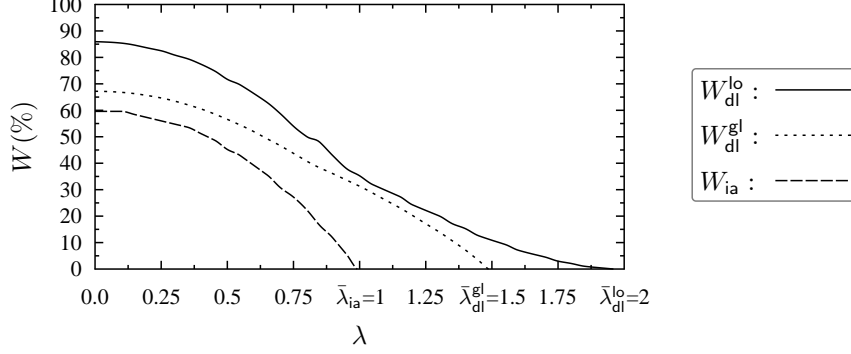
Figure 5: W(\lambda, \pi) for isolated agents and for decentralized learning from others with locally and globally determined reputations. f_X = 1 and \pi = 1/2 such that \bar{\lambda}_{ia} = 1 , \bar{\lambda}_{dl}^{gl} = 3/2 , and \bar{\lambda}_{dl}^{lo} = 2 .
