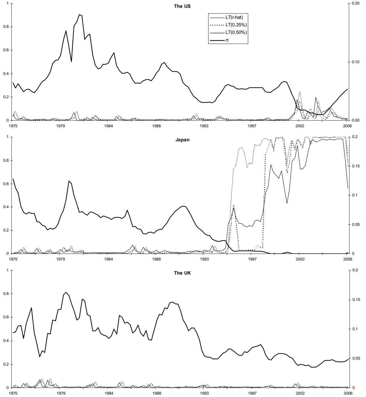
Figure 6: In each panel is plotted: the estimated probability of LT (Left hand scale) when r is estimated, LT(r\text{-hat}) ; the estimated probabilities of LT when r = 0.25\% and 0.5\% , LT(0.25\%) and LT(0.50\%) ; and the interest rate, rt (Right hand scale).
